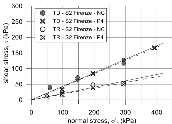
Figure 4. Direct shear test and anular shear test results for samples before (NC) and after the conditioning process with product P4.
